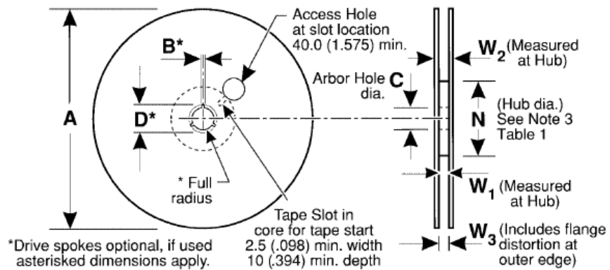
Figure 3: Reel Dimensions (Metric Dimensions will govern)
