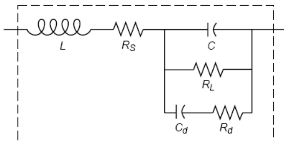
FIGURE 8 The Real Capacitor
