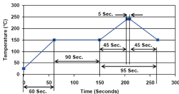
FIGURE 13 Time/Temperature Soldering Profile
