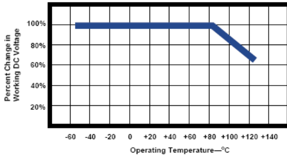
FIGURE 3 Working DC Voltage Change with Temperature
