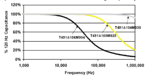
FIGURE 1 Typical Effect of Frequency upon Capacitance
