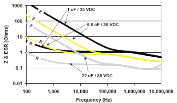
FIGURE 9a ESR & Impedance (Z) vs Frequency
