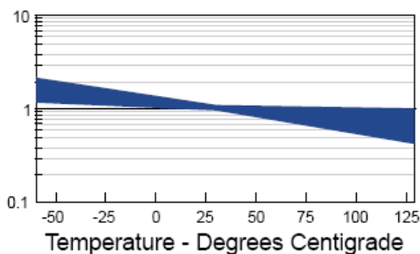
FIGURE 10 Typical Effect of Temperature on 100 kHz ESR
