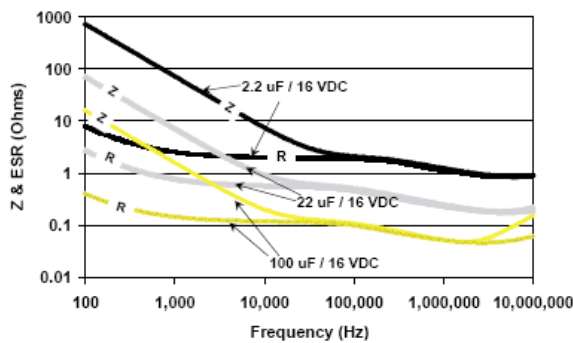
FIGURE 9b ESR & Impedance (z) vs Frequency
