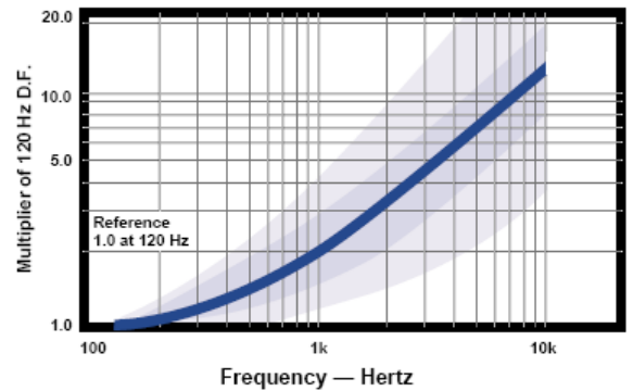
FIGURE 6 Typical Effect of Frequency upon Dissipation Factor
