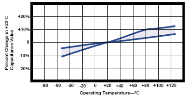
FIGURE 2 Typical Effect of Temperature upon Capacitance
